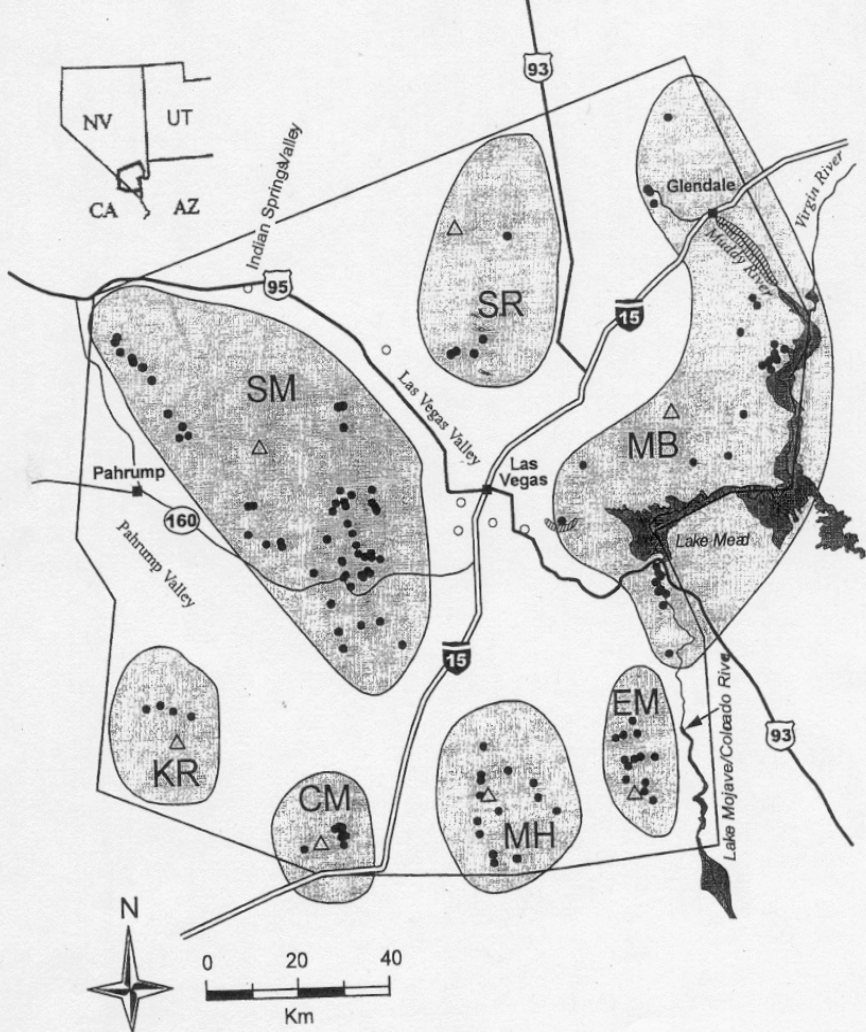
Fig. 1. Study area (outline) and sites surveyed for amphibians in the eastern Mojave Desert. Closed circles indicate sites in the Upland Springs Survey ( n = 128 ). Shaded areas represent mountain range groups: CM = Clark Mountain Range, EM = Eldorado Mountains, KR = Kingston Range, MB = Muddy and Black Mountains, MH = McCullough and Highland Ranges, SM = Spring Mountains, SR = Sheep Range. High point in each mountain range group is indicated by a triangle. The Lowland Records Review and Survey included sites within the Las Vegas, Pahrump, and Indian Springs valleys; floodplains of the Muddy River and the former Colorado and Virgin Rivers (now submerged by Lakes Mead and Mojave); and shorelines of Lakes Mead and Mojave. Sites surveyed for amphibians in these areas are depicted by cross-hatching (Las Vegas Wash and Muddy River) and open circles.
